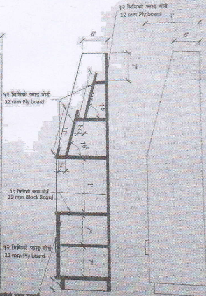
कटर हेरेको मोहोडा (side Sectional View at A-A)
